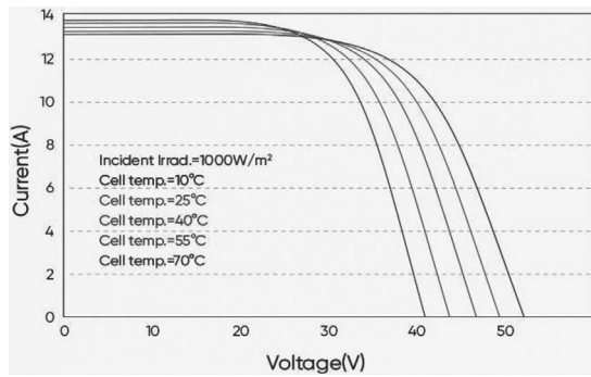
1-V Curve at Different Temperature (SSSW)
