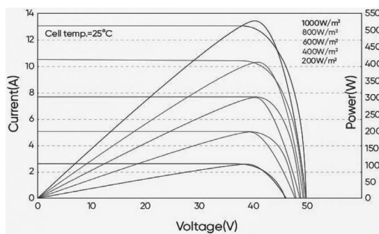
1-V / P - V Curve at Different Temperature (SSSW)
