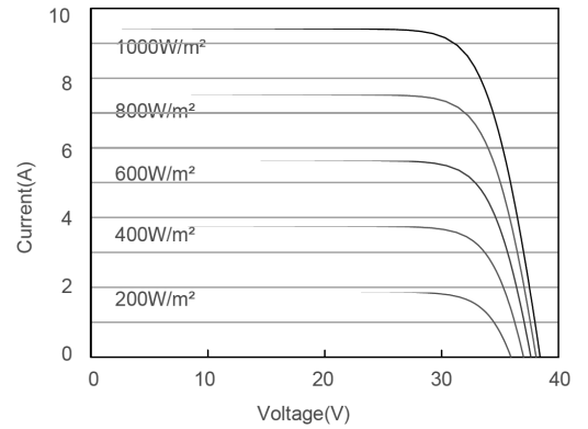
Current-Voltage Curve
