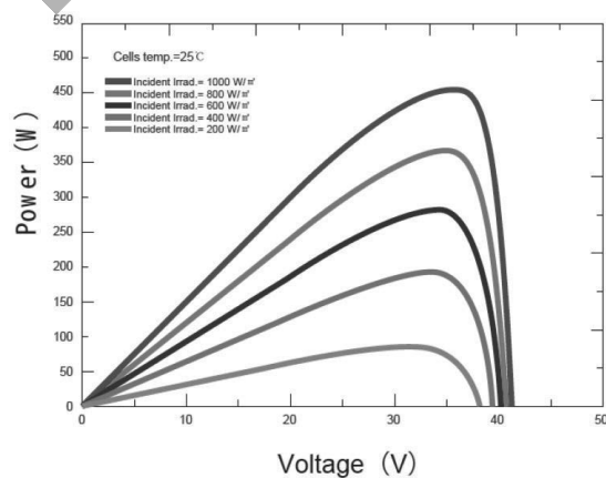
P-V Curve at Different Irradiance(450W)
