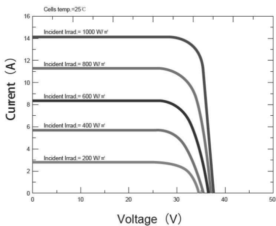
I-V Curve at Different Irradiance(450W)
